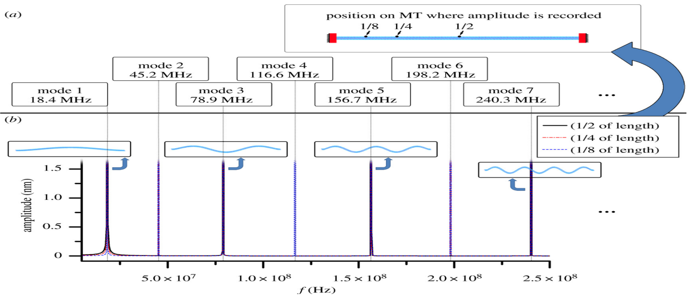
Mechanical Vibrational Frequencies of Microtubules
